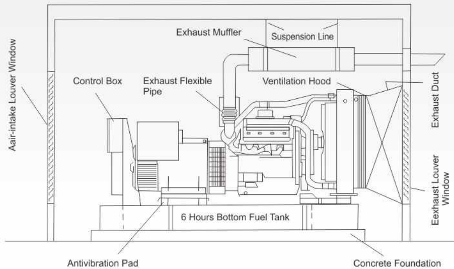
Standard Installing Designs(Profile)
