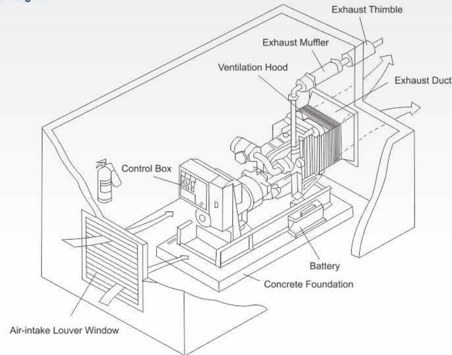
Standard Installing Designs(Profile)
